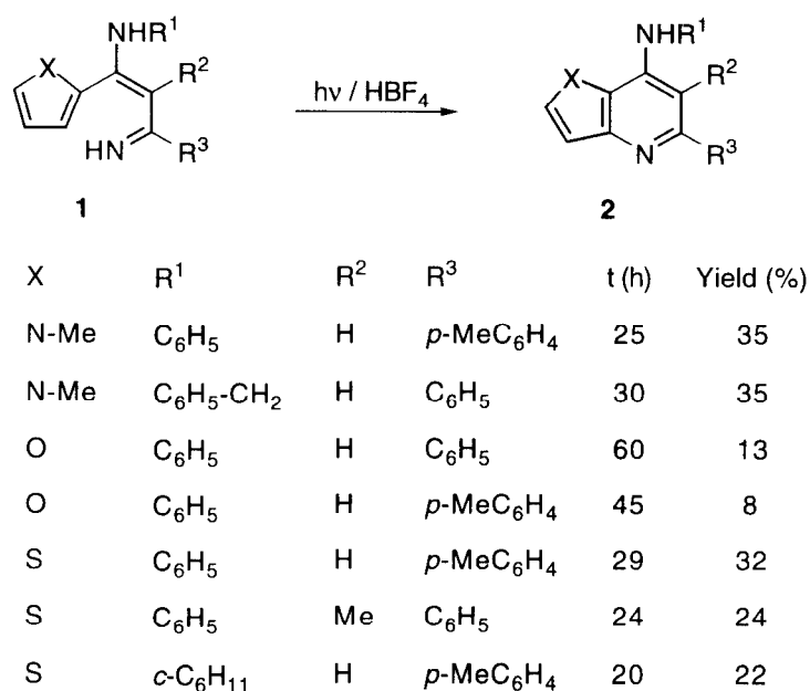
Scheme 1
