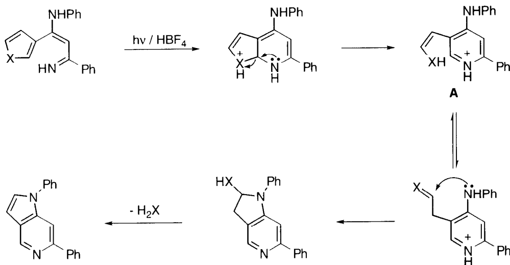
Scheme 6
