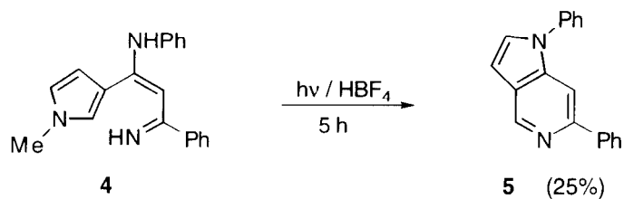
Scheme 3
