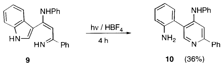
Scheme 7
